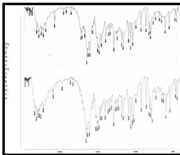
Fig. 2: FTIR spectra of pure Capecitabine and Capecitabine loaded nano particles formulation (FN4)
